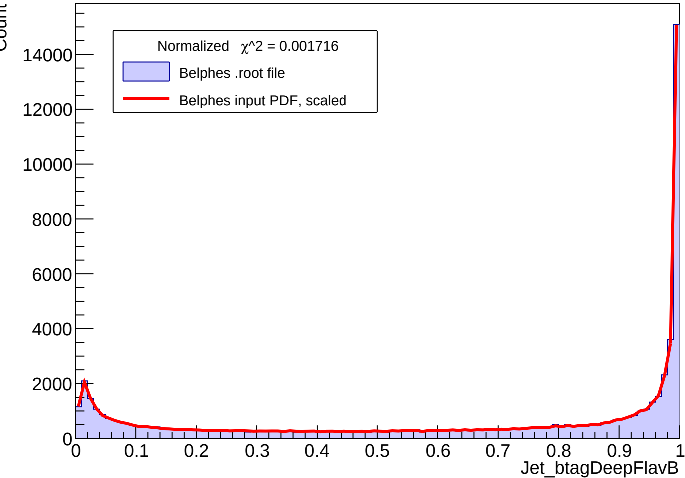
Jet_btagDeepFlavB on PT={30.0, 40.0}, abs(Eta)={0.0, 0.5}
